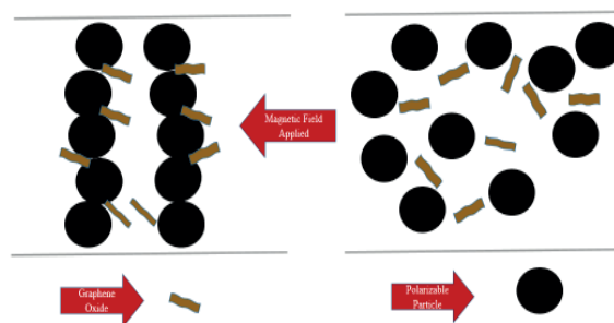
Fig.1. Schematic diagram of GO based MR fluid
