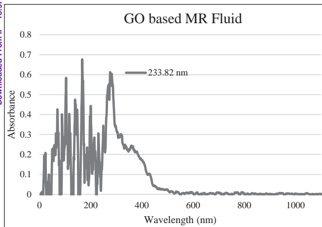
Fig.4. Absorption spectrum of GO based MR fluid
