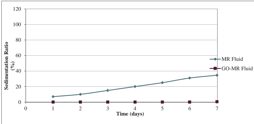
Fig.6. Sedimentation rate of MR fluids
