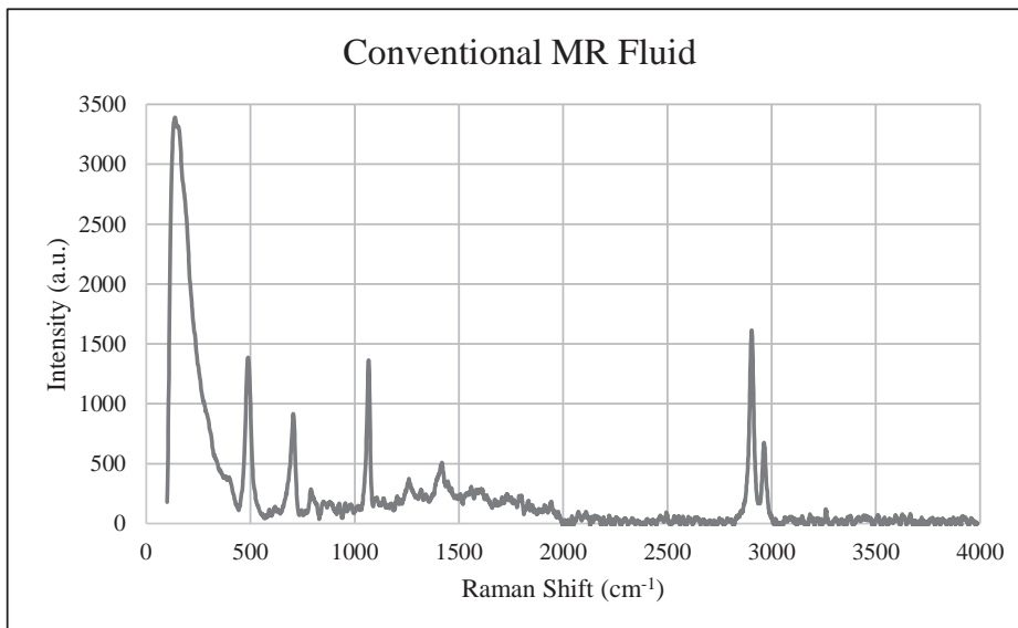
Fig.2. Raman spectrum of Conventional MR fluid
