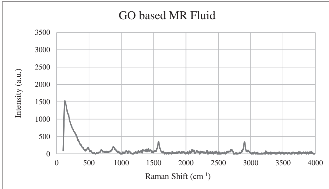
Fig.3. Raman spectrum of GO based MR fluid
