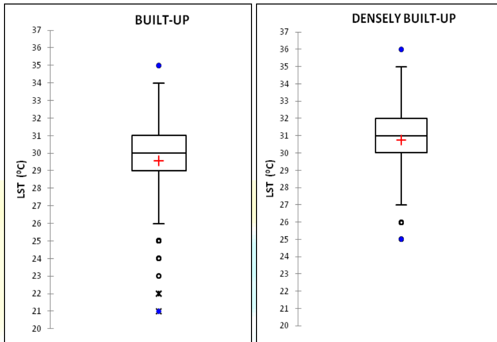
Figure 6: Boxplot of LST by land cover types
