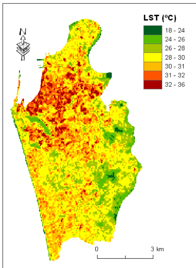
Figure 3: Land surface temperature in Colombo retrieved from March 14, 2001
