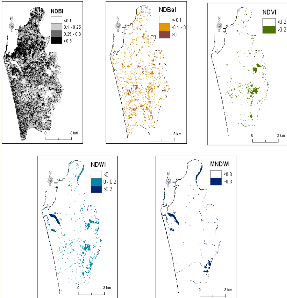
Figure 4: NDBI, NDBaI, NDVI, NDWI and MNDWI indices in Colombo derived from March 14, 2001Landsat ETM+ image
