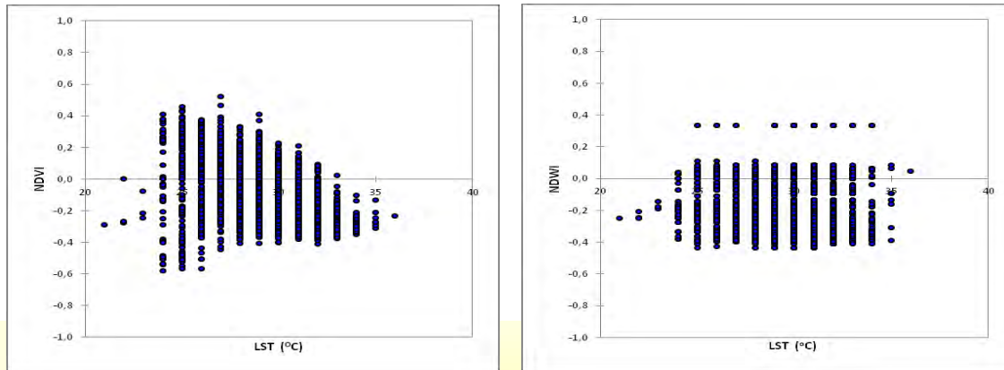
Figure 5: Scatterplot of the LST-NDBI, LST-NDBaI, LST-NDVI, LST-NDWI feature space
