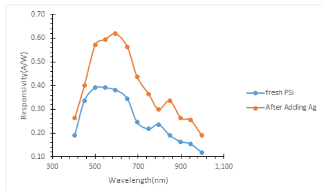
Figure 6: Responsivity before and after adding Ag
