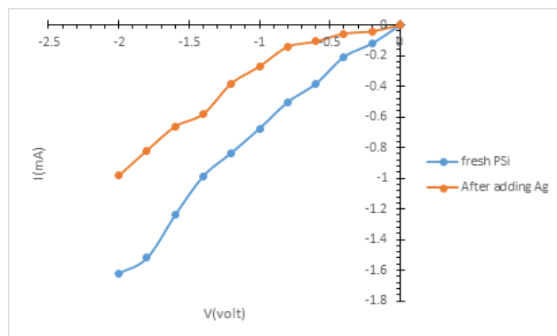
Figure 5: behavior of I-V characteristics before and after depositing Ag nanoparticle in illumination
