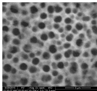
Figure 1: SEM image for fresh PSi.
