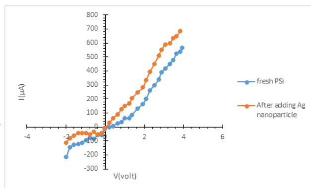
Figure 4: behavior of I-V characteristics before and after adding Ag nanoparticle in dark
