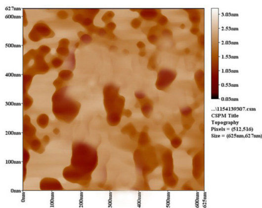
Figure 3. 2D AFM image a) fresh porous silicon b) after adding Ag nanoparticle
