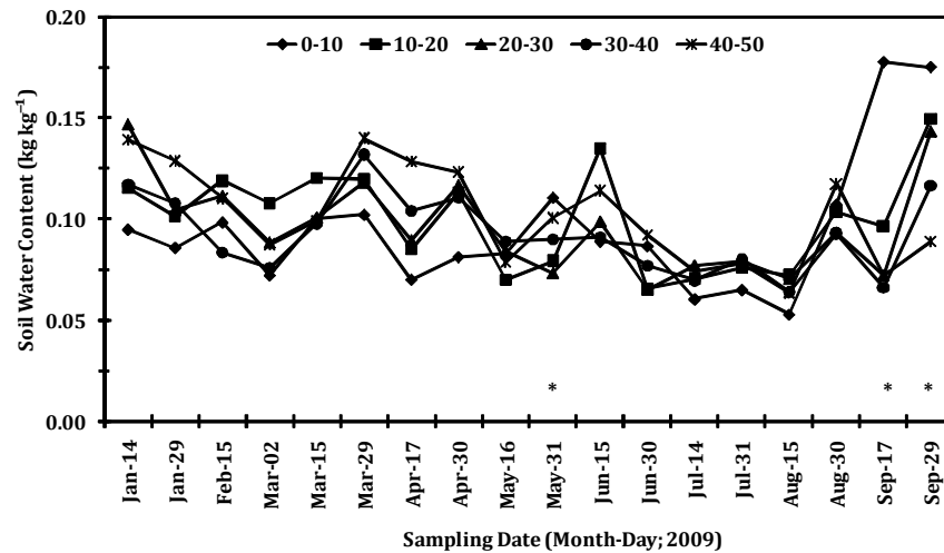
Figure 2: Seasonal variation in gravimetric soil water content at five soil profile depths (cm) at the research site. For a given sampling date, statistically significant probabilities ( p < 0.05 ) according to one-way ANOVA are shown in asterisk (*)
