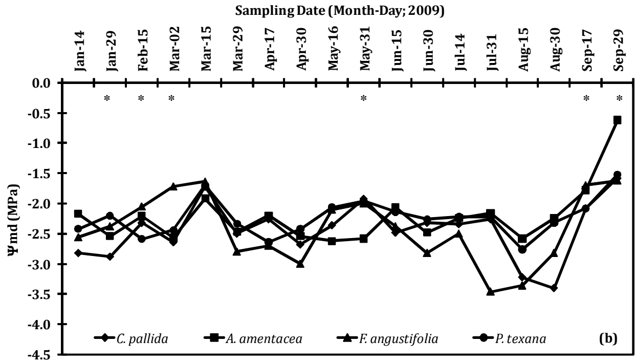
Figure 3: Seasonal variation in pre-dawn (a) and mid-day (b) xylem water potential in four shrub species. For a given sampling date, statistically significant probabilities ( p \leq 0.05 ) according to the Kruskal-Wallis test are shown in asterisk (*)
